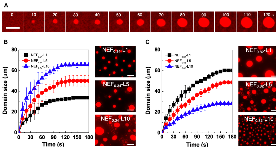
Fig. 3. Phase separation kinetics of NEFs. (A) Time-lapse fluorescence images of the coarsening oil domain of NEF 0.34 -L5 at 80°C. Scale bar, 50 \mu\text{m} . Phase separation kinetics of NEFs depending on the number of layers: (B) NEF 0.34 and (C) NEF 0.82 . Fluorescence images were obtained after full decomposition. Scale bars, 50 \mu\text{m} . In the NEF \phi -L \alpha , \phi is the oil mass fraction in the NEF, and \alpha is the number of layers.
