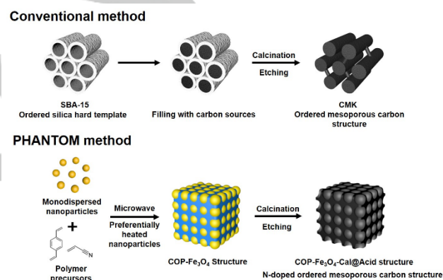
Scheme 1. Microwave heating for preferential assembly. Comparison of a conventional synthetic route with preferential heating and assembly for nanoparticle templated ordered mesoporous materials (PHANTOM) method.
